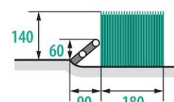
11 ANGIELSKI SKOK DITCH AND HEDGE
