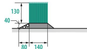
11 ANGIELSKI SKOK DITCH AND HEDGE
